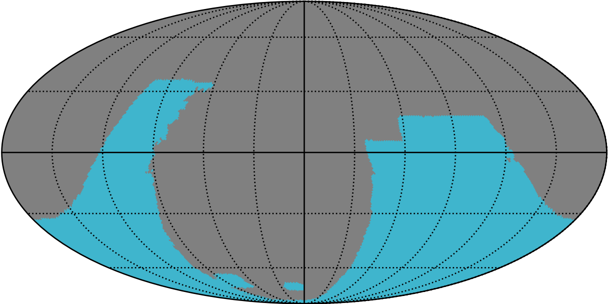
weather_cloudso4v3.4_10yrs : GalplaneFootprintMetric_galactic_plane_map_Tau_2_0
