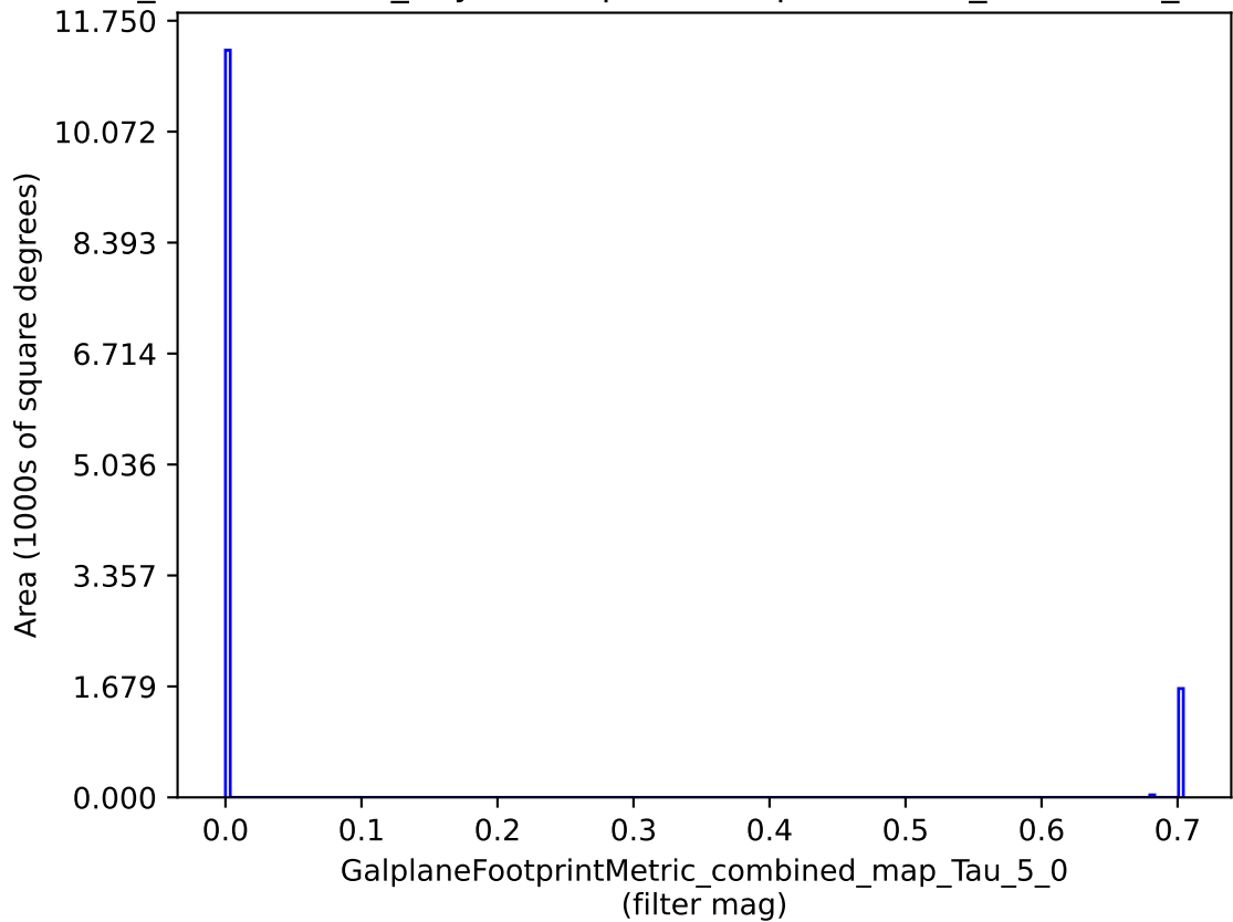
weather_cloudso4v3.4_10yrs : GalplaneFootprintMetric_combined_map_Tau_5_0
