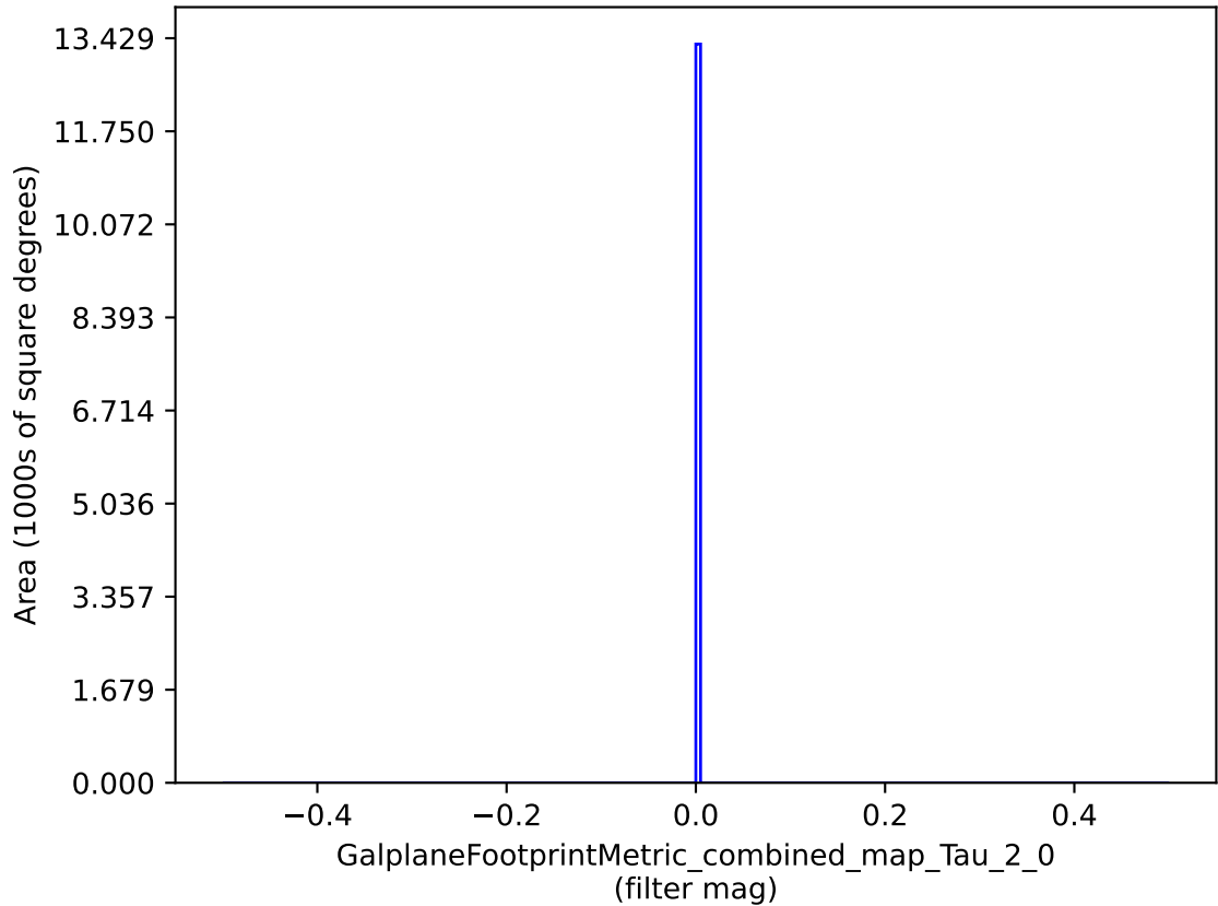
weather_cloudso4v3.4_10yrs : GalplaneFootprintMetric_combined_map_Tau_2_0
