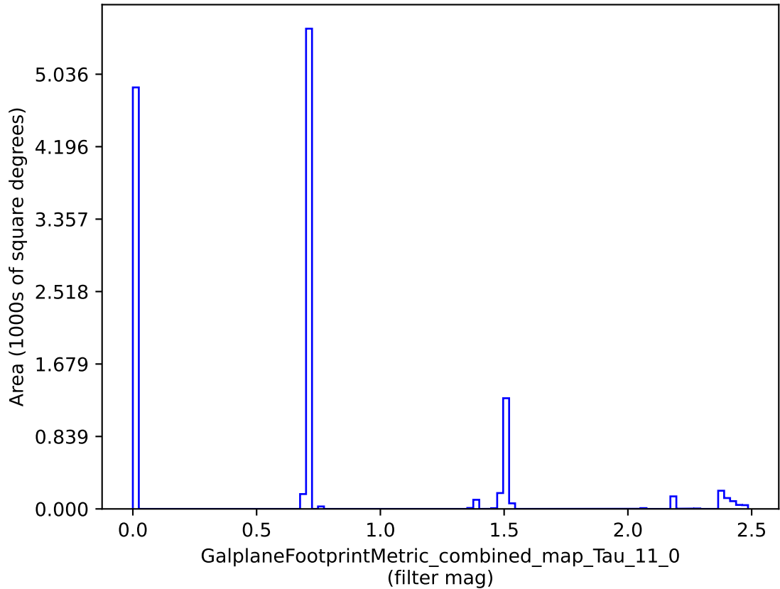
weather_cloudso4v3.4_10yrs : GalplaneFootprintMetric_combined_map_Tau_11_0
