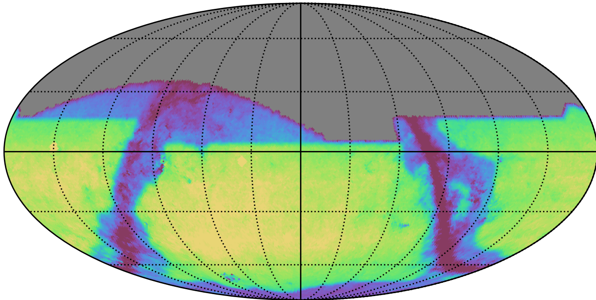
weather_cloudso4v3.4_10yrs z: GalaxyCountsMetricExtended
