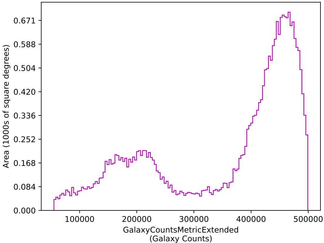
weather_cloudso4v3.4_10yrs z: GalaxyCountsMetricExtended
