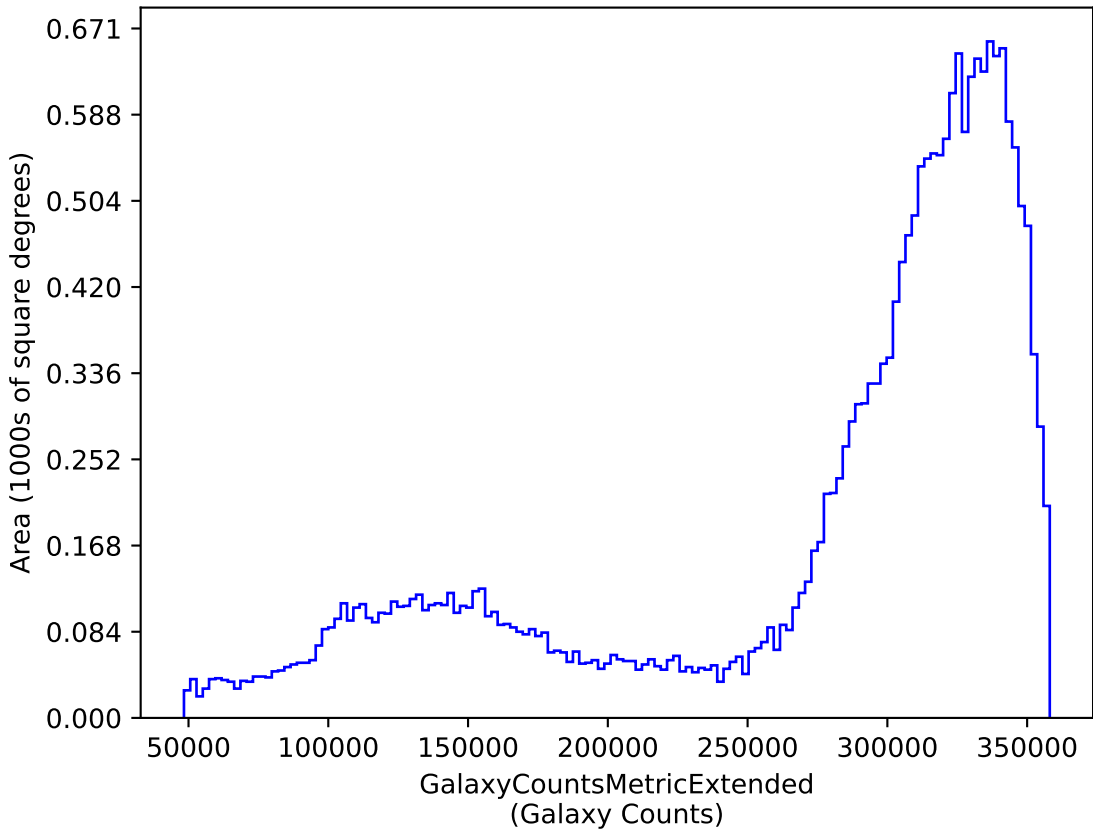
weather_cloudso4v3.4_10yrs y: GalaxyCountsMetricExtended
