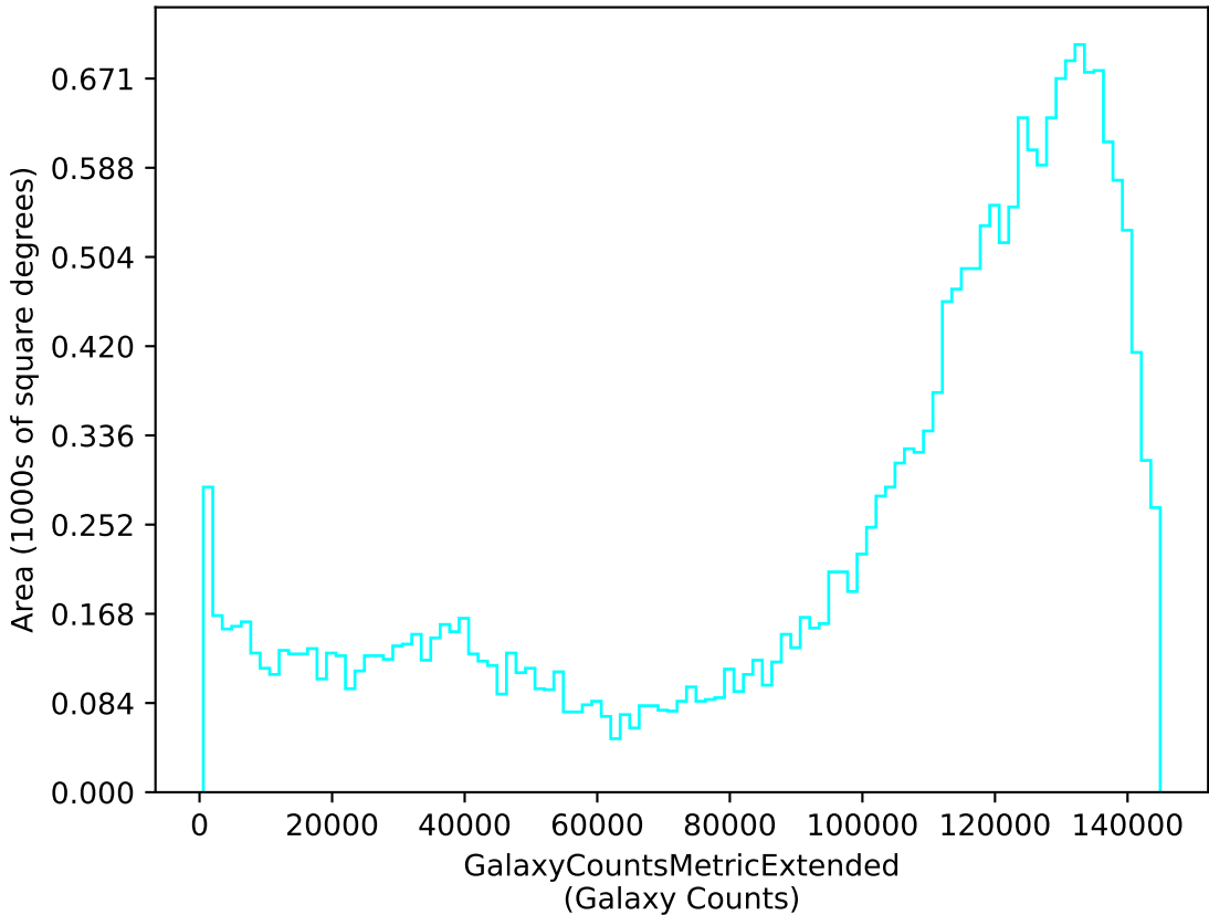
weather_cloudso4v3.4_10yrs u: GalaxyCountsMetricExtended
