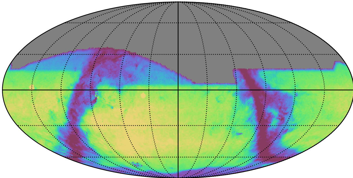
weather_cloudso4v3.4_10yrs r: GalaxyCountsMetricExtended
