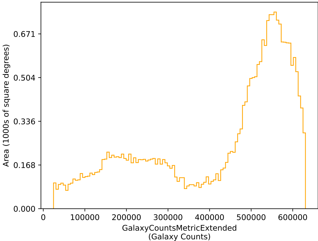
weather_cloudso4v3.4_10yrs r: GalaxyCountsMetricExtended
