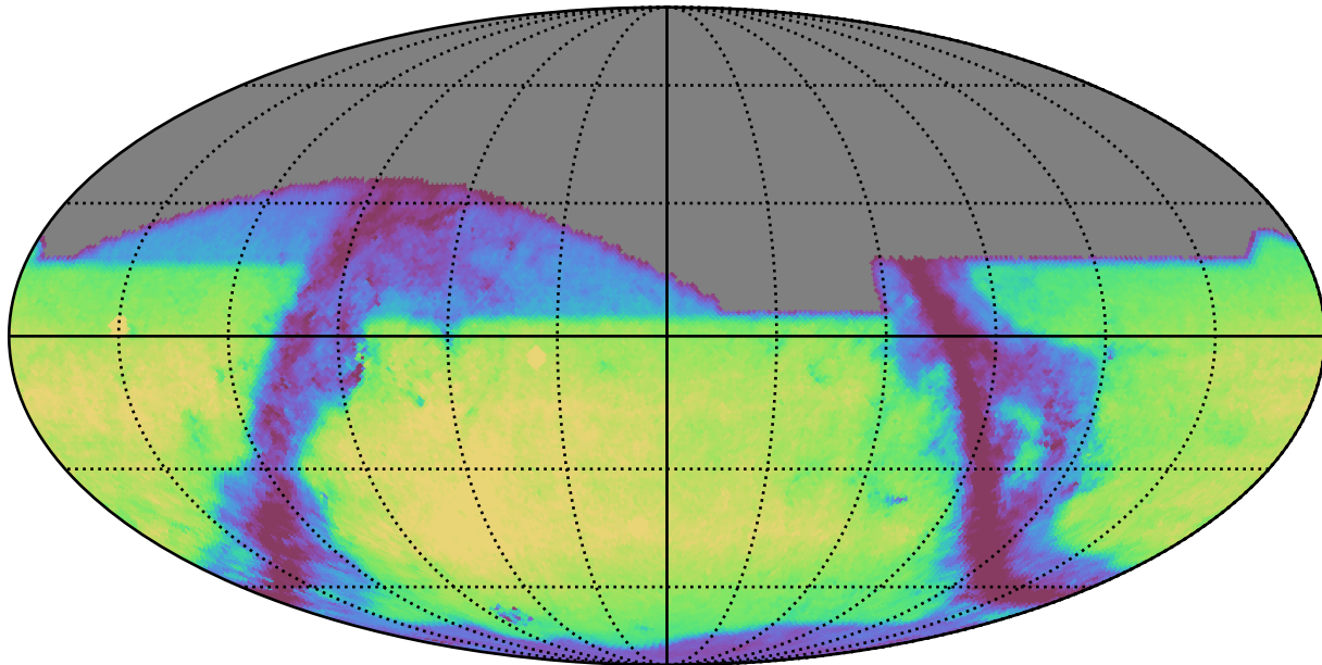
weather_cloudso4v3.4_10yrs i: GalaxyCountsMetricExtended
