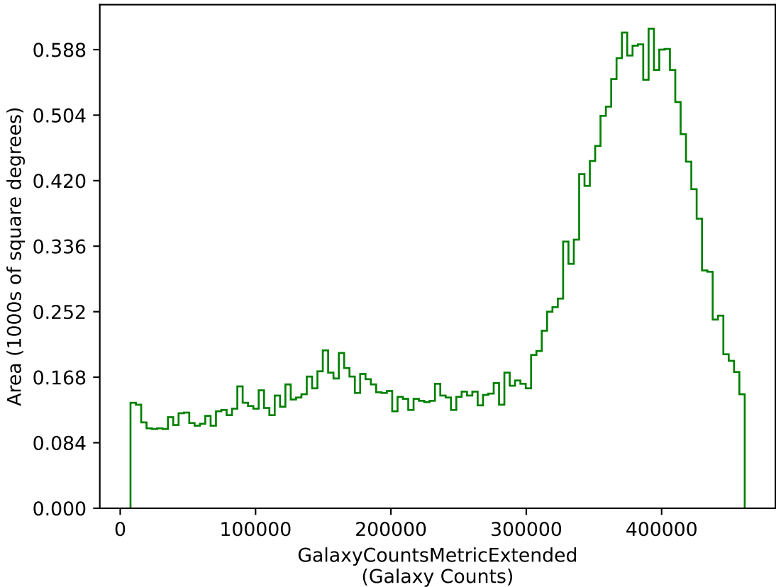
weather_cloudso4v3.4_10yrs g: GalaxyCountsMetricExtended
