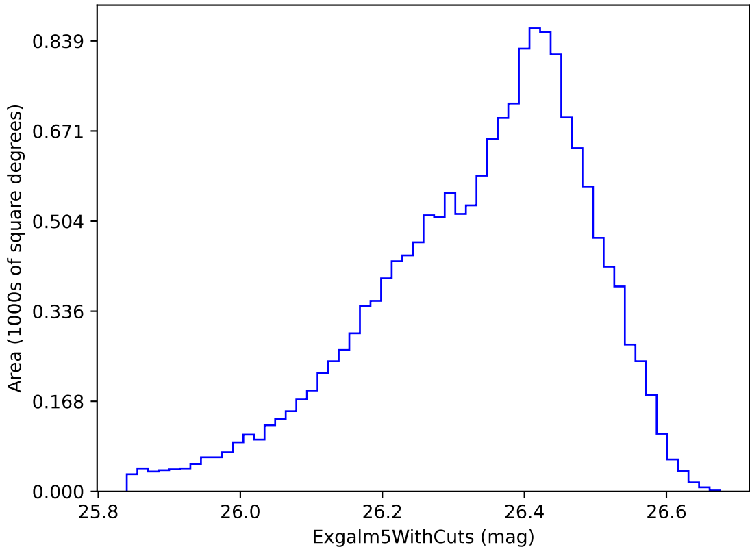
weather_cloudso4v3.4_10yrs i band non-DD year 9: Exgalml5WithCuts
