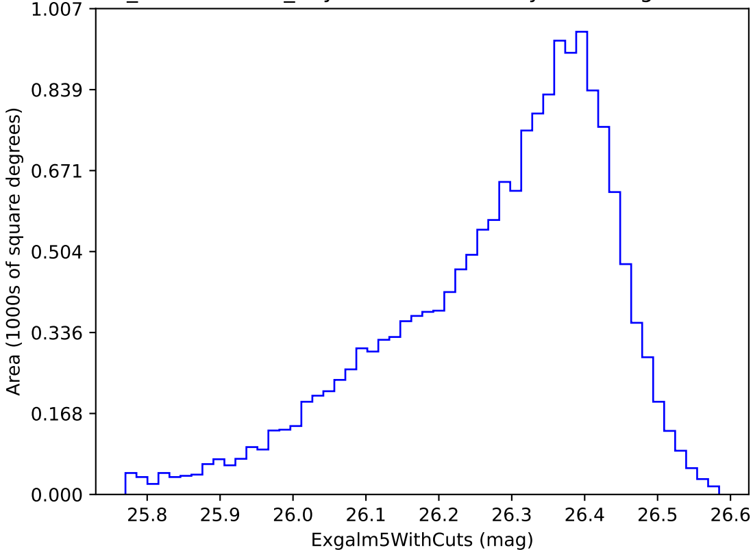
weather_cloudso4v3.4_10yrs i band non-DD year 8: ExgalM5WithCuts
