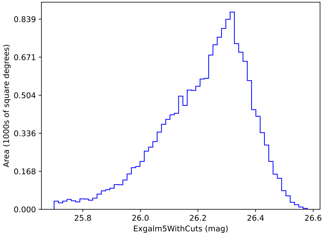
weather_cloudso4v3.4_10yrs i band non-DD year 7: Exgalml5WithCuts
