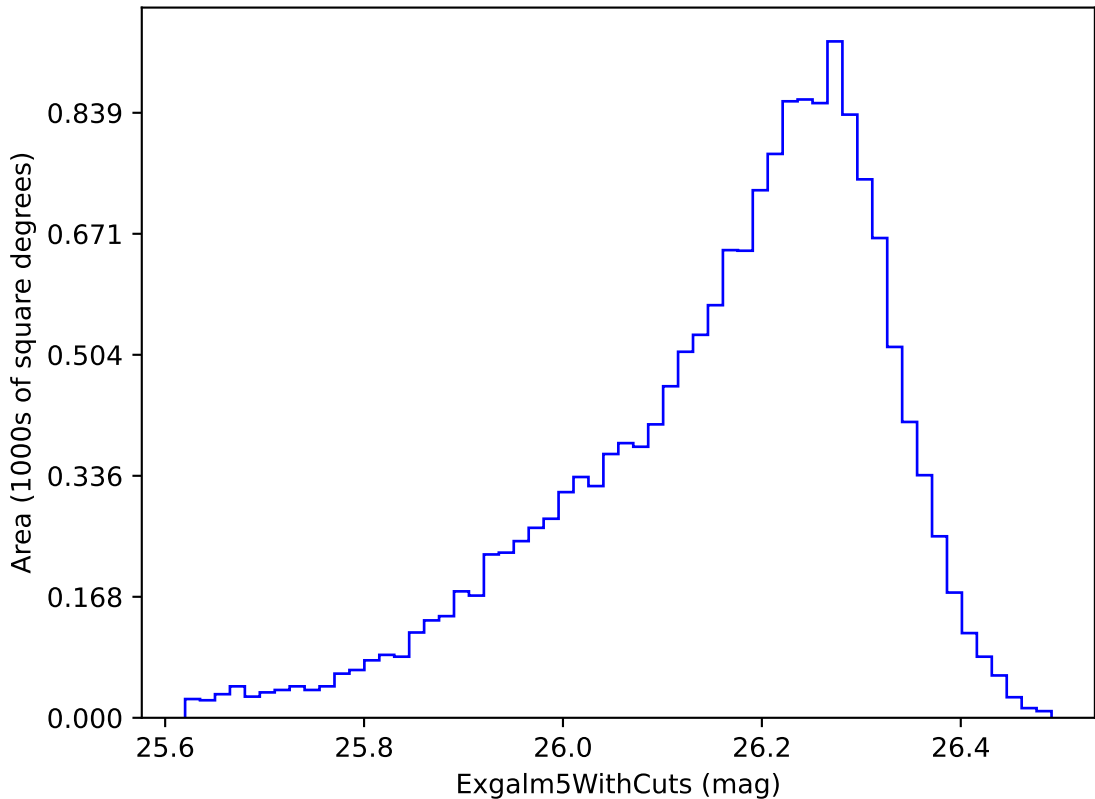
weather_cloudso4v3.4_10yrs i band non-DD year 6: ExgalM5WithCuts
