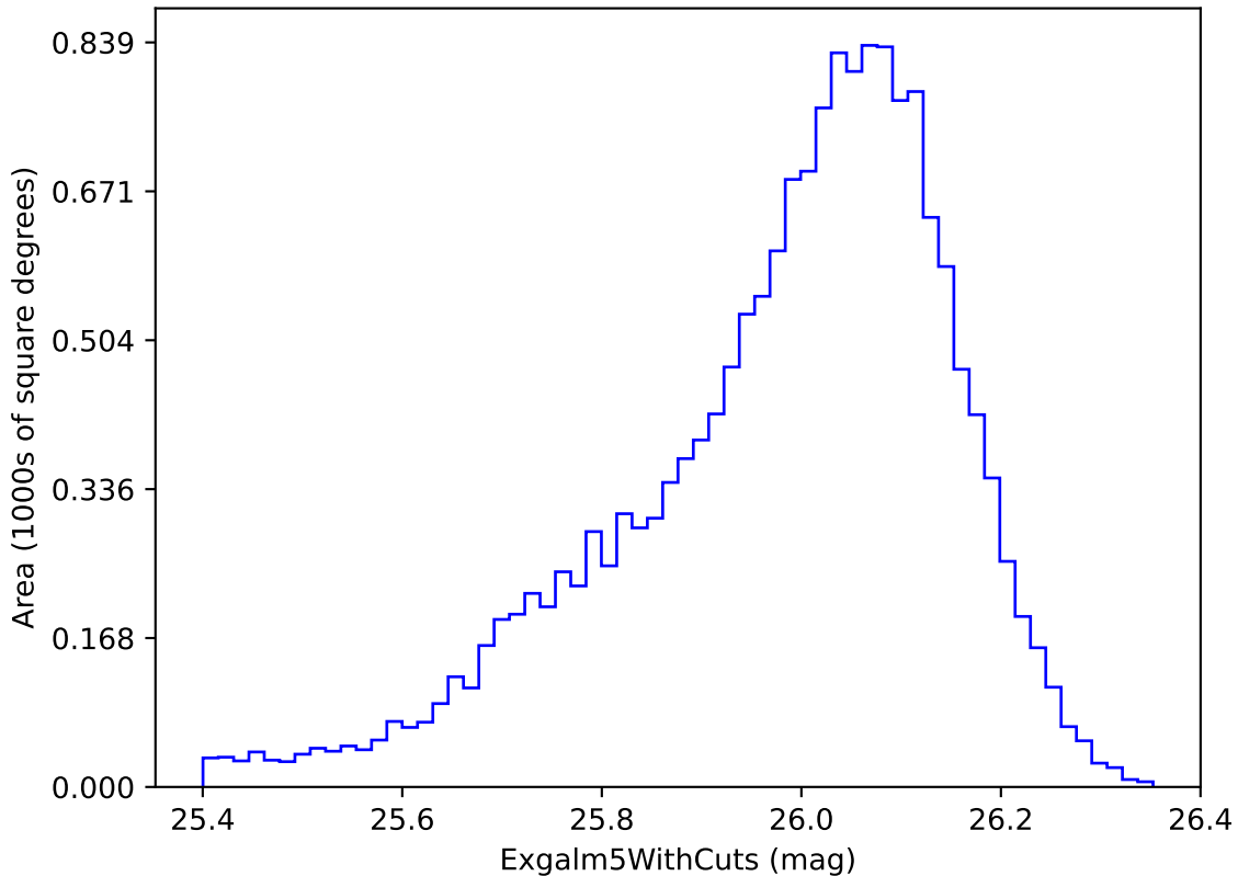
weather_cloudso4v3.4_10yrs i band non-DD year 4: Exgal5WithCuts
