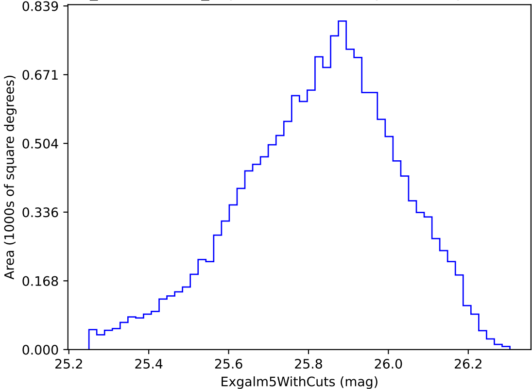
weather_cloudso4v3.4_10yrs i band non-DD year 3: Exgalml5WithCuts
