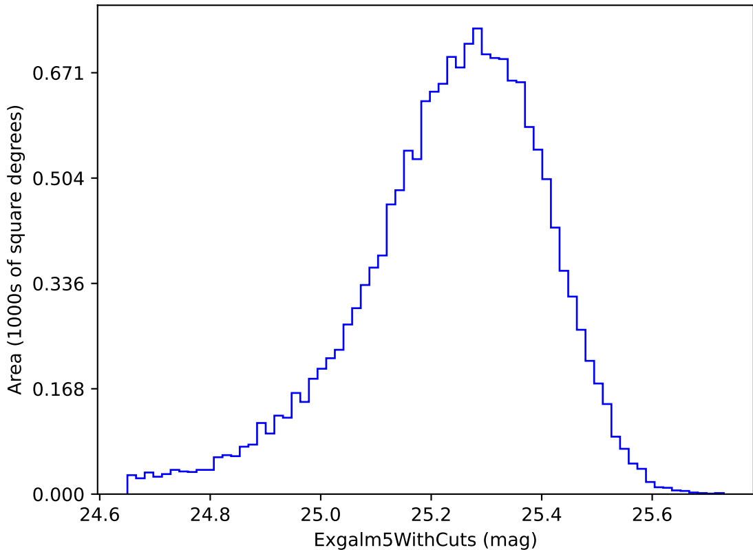
weather_cloudso4v3.4_10yrs i band non-DD year 1: Exgalml5WithCuts
