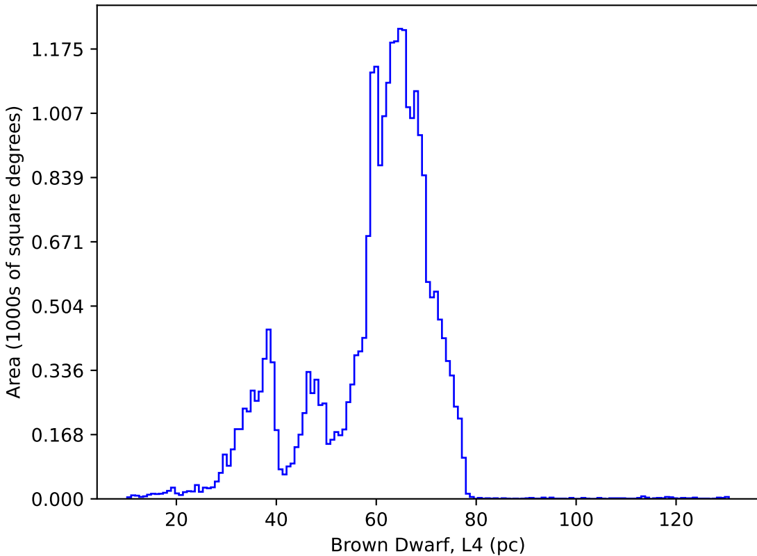
weather_cloudso4v3.4_10yrs : Brown Dwarf, L4
