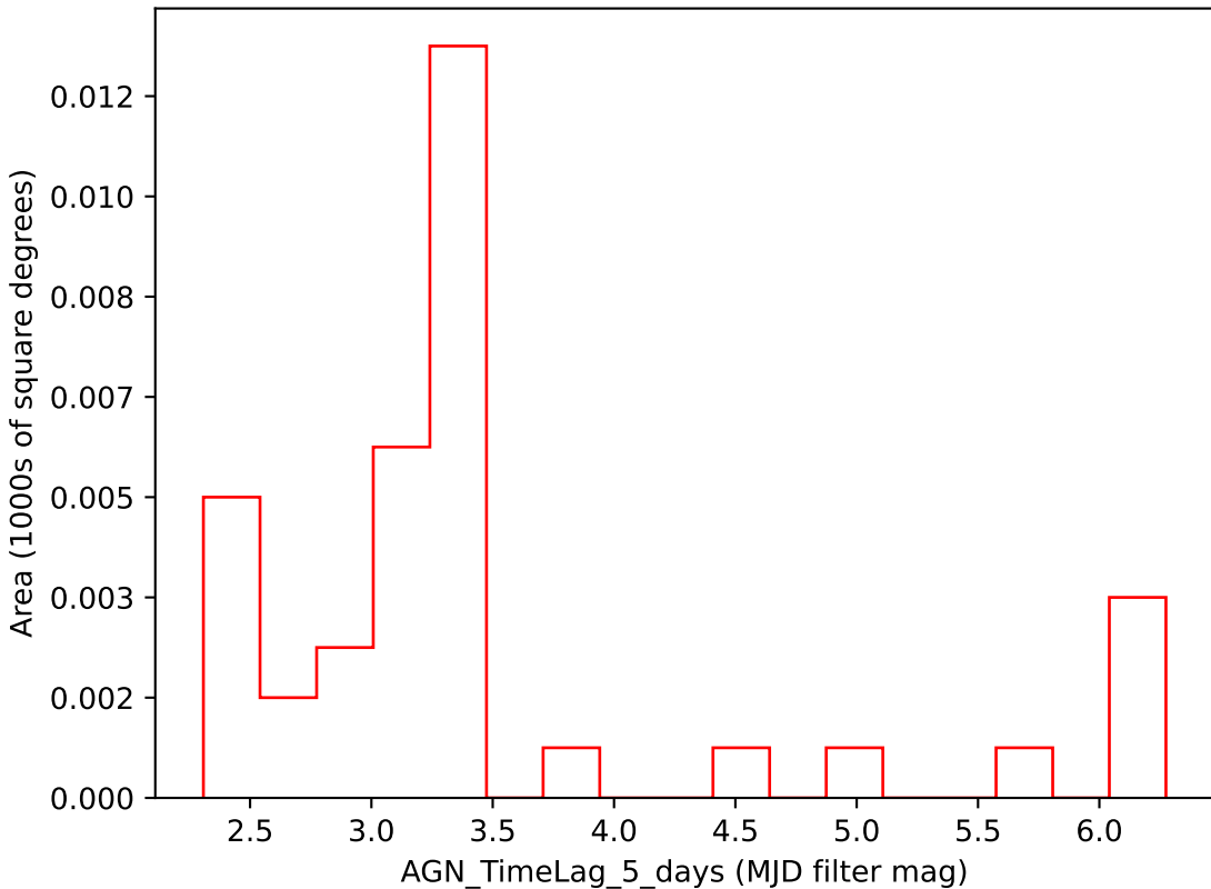
weather_cloudso4v3.4_10yrs i band: AGN_TimeLag_5_days
