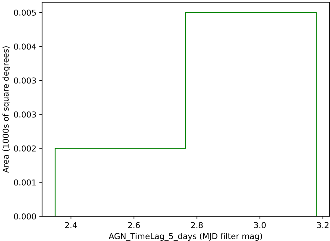
weather_cloudso4v3.4_10yrs g band: AGN_TimeLag_5_days
