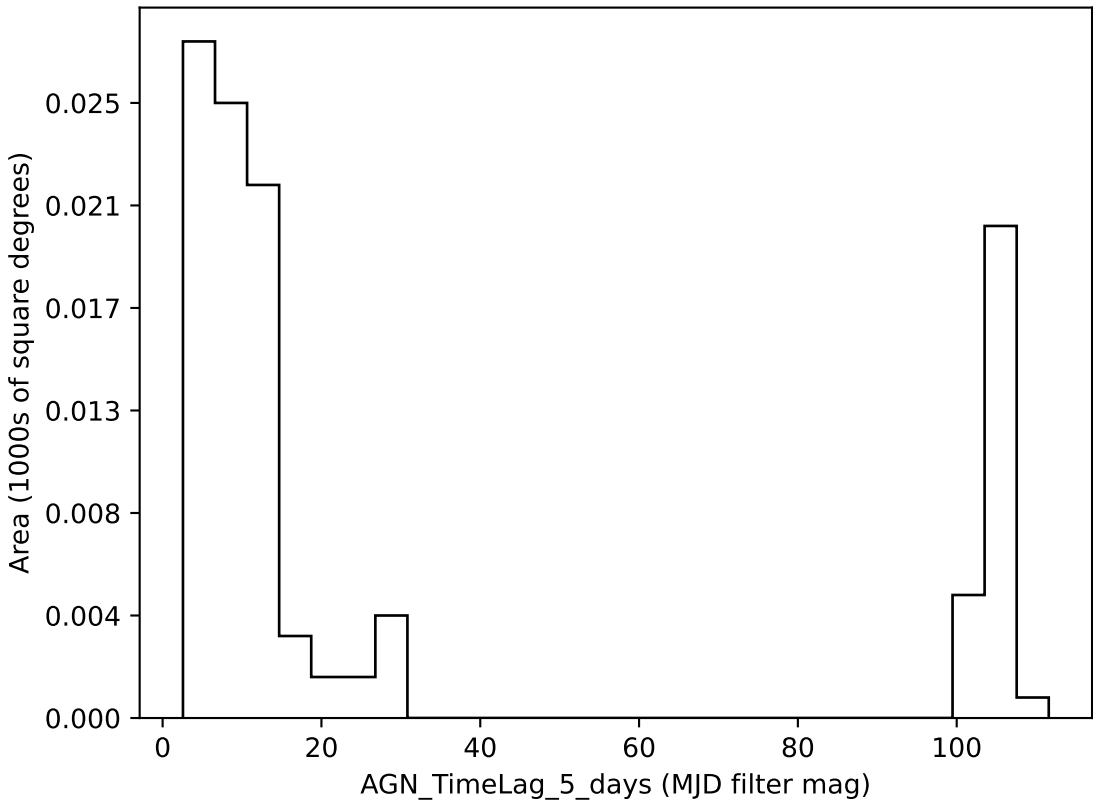
weather_cloudso4v3.4_10yrs all bands: AGN_TimeLag_5_days
