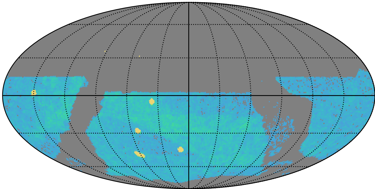
weather_cloudso4v3.4_10yrs z band: AGN_TimeLag_100_days
