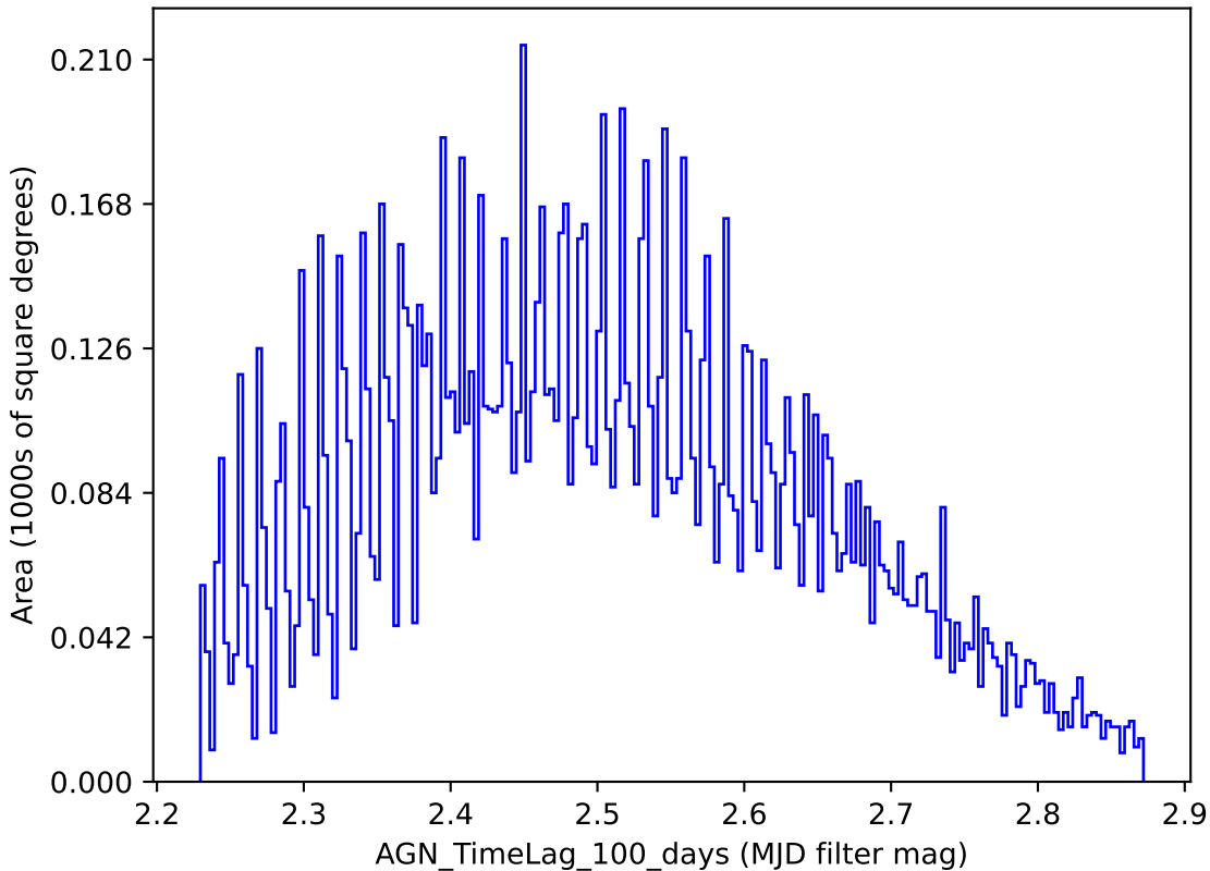
weather_cloudso4v3.4_10yrs y band: AGN_TimeLag_100_days
