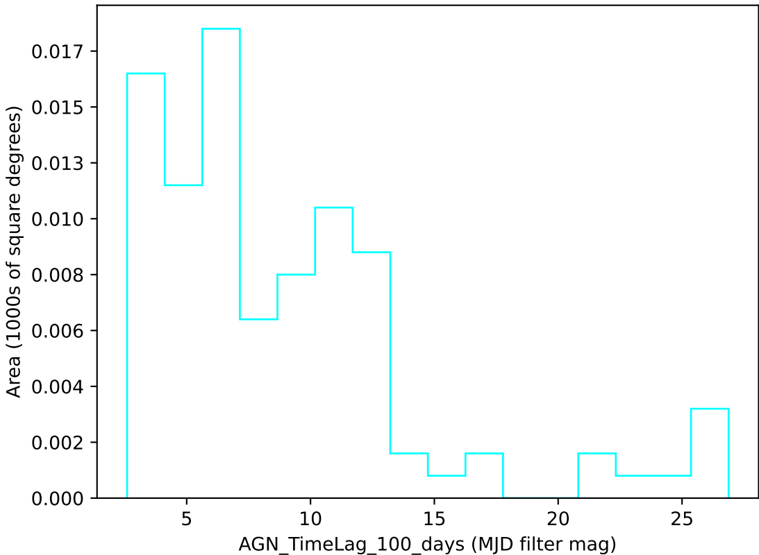
weather_cloudso4v3.4_10yrs u band: AGN_TimeLag_100_days
