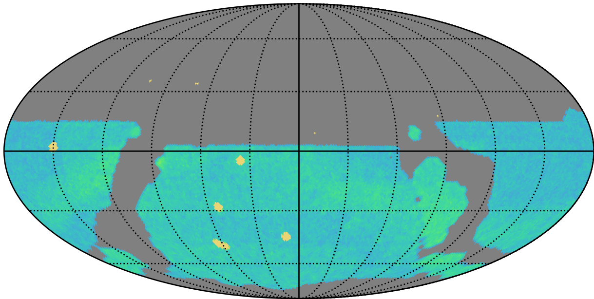
weather_cloudso4v3.4_10yrs r band: AGN_TimeLag_100_days
