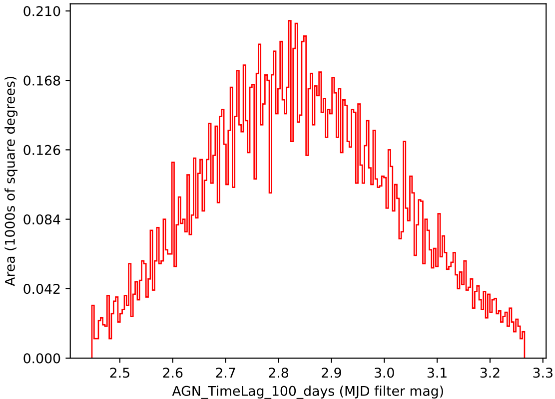
weather_cloudso4v3.4_10yrs i band: AGN_TimeLag_100_days
