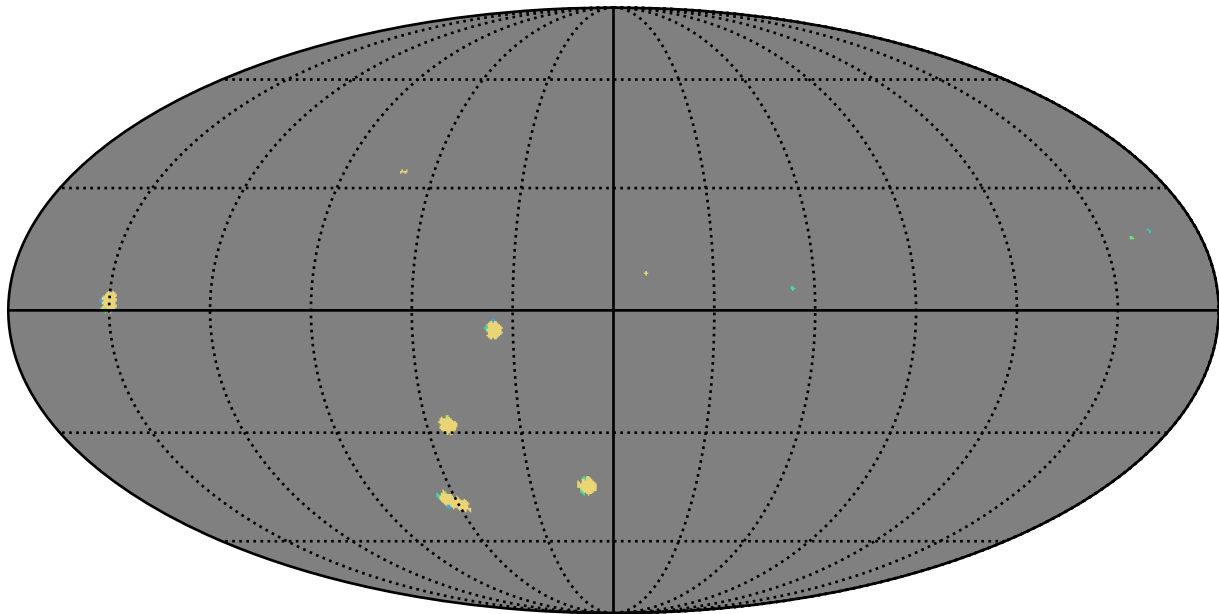
weather_cloudso4v3.4_10yrs g band: AGN_TimeLag_100_days
