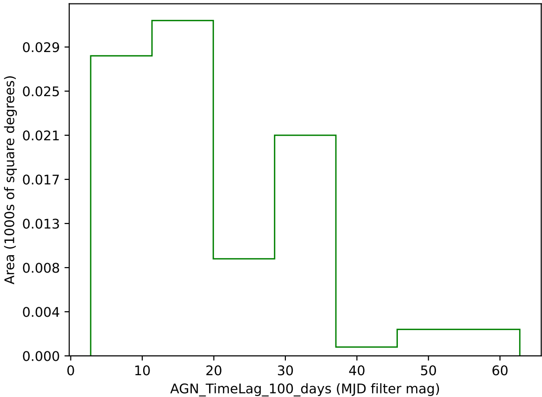
weather_cloudso4v3.4_10yrs g band: AGN_TimeLag_100_days
