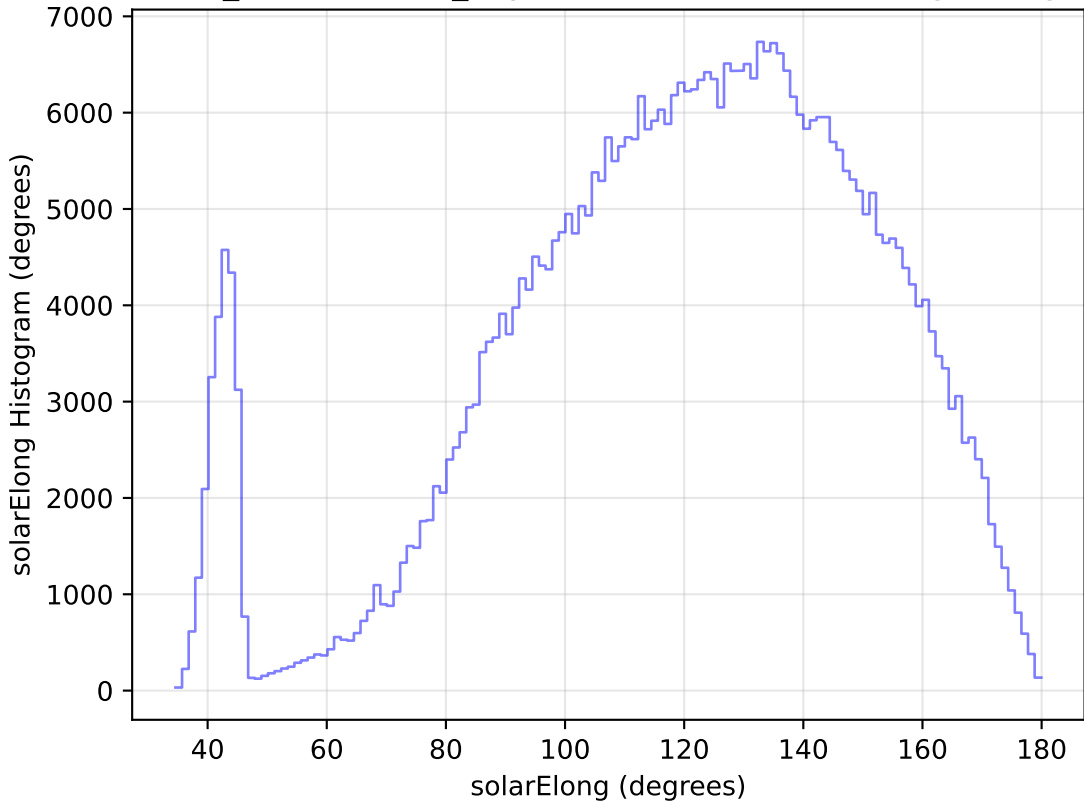
weather_cloudso4v3.4_10yrs WFD z band: solarElong Histogram
