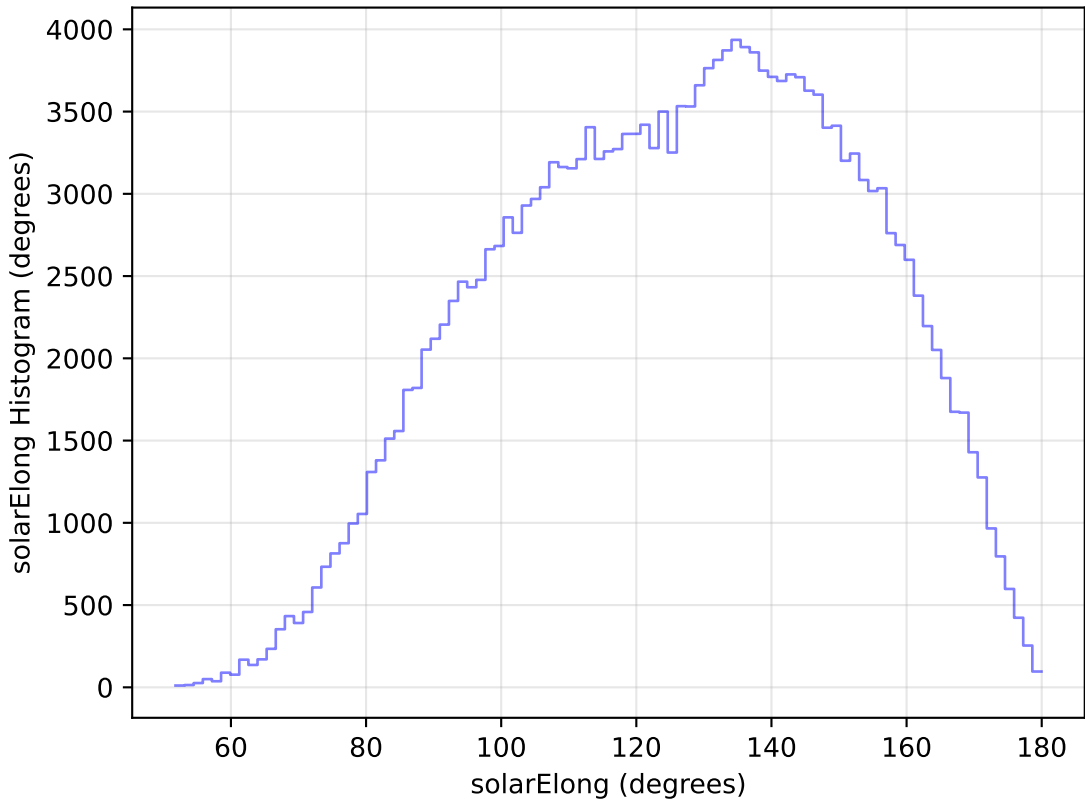
weather_cloudso4v3.4_10yrs WFD g band: solarElong Histogram
