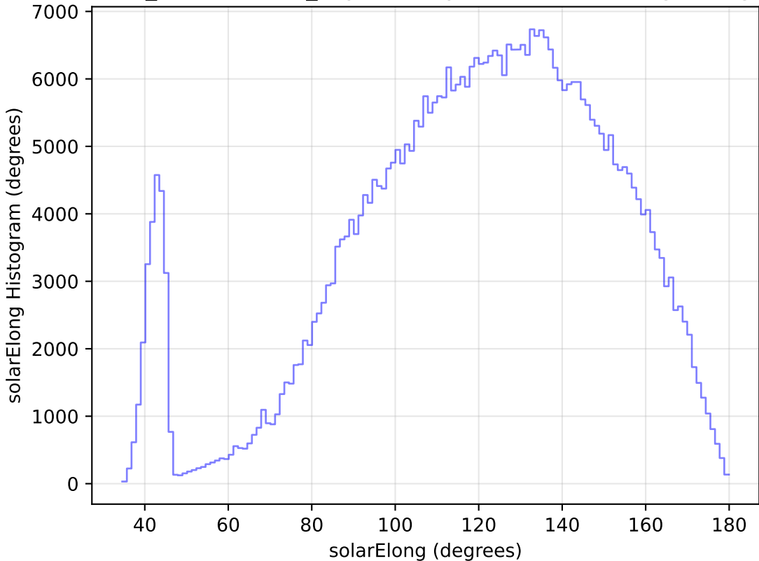
weather_cloudso4v3.4_10yrs All sky z band: solarElong Histogram
