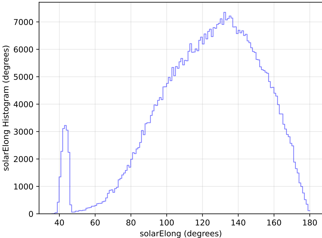
weather_cloudso4v3.4_10yrs All sky r band: solarElong Histogram
