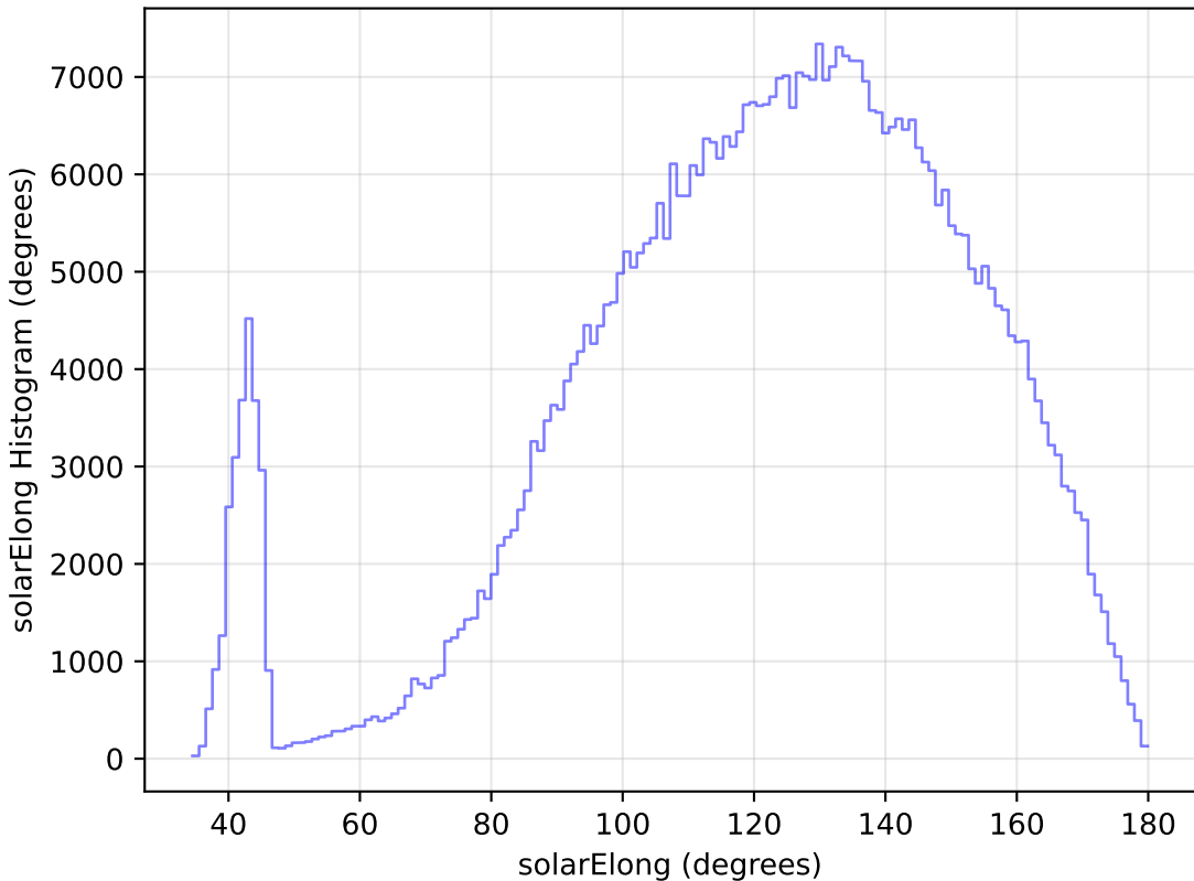
weather_cloudso4v3.4_10yrs All sky i band: solarElong Histogram
