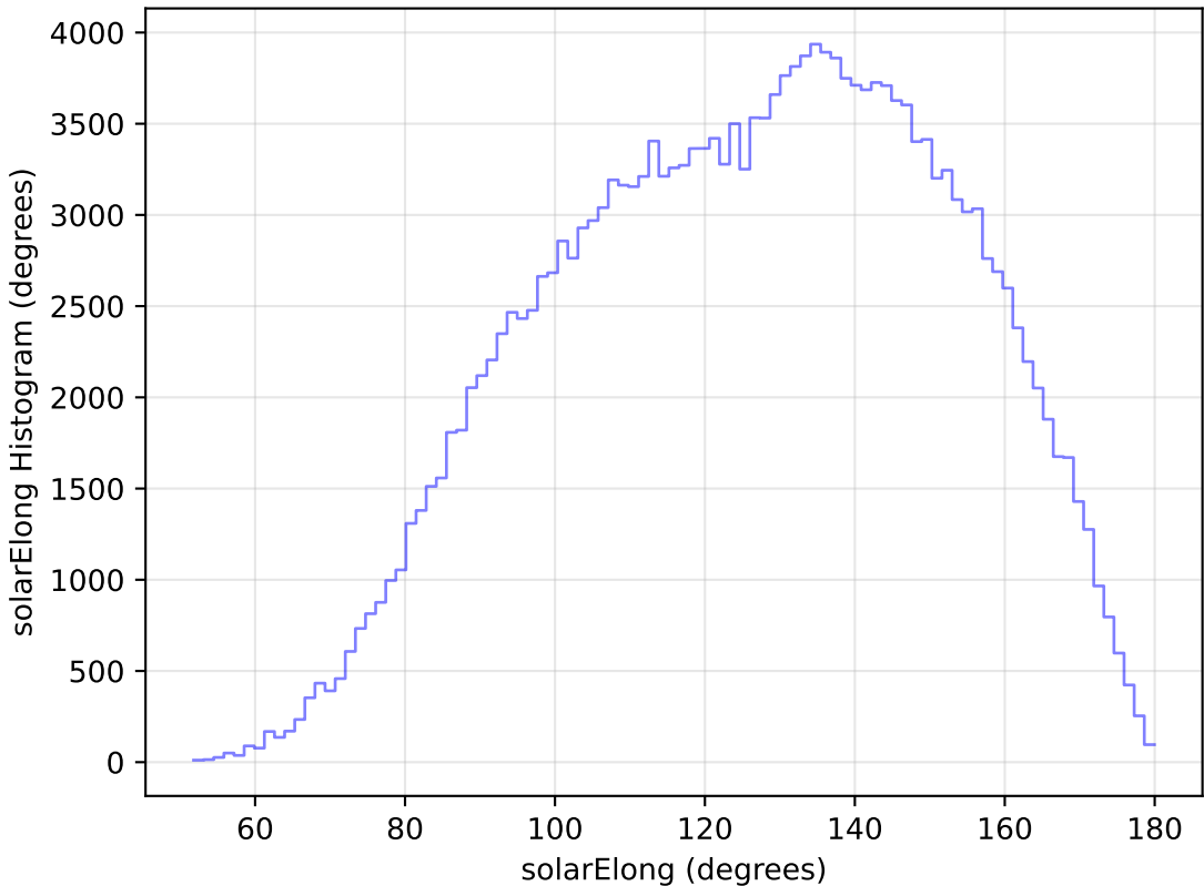
weather_cloudso4v3.4_10yrs All sky g band: solarElong Histogram
