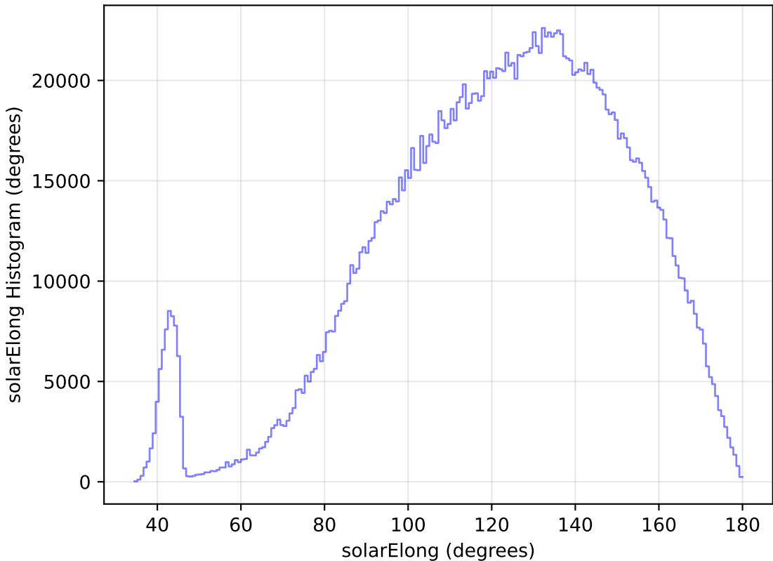
weather_cloudso4v3.4_10yrs All sky all bands: solarElong Histogram
