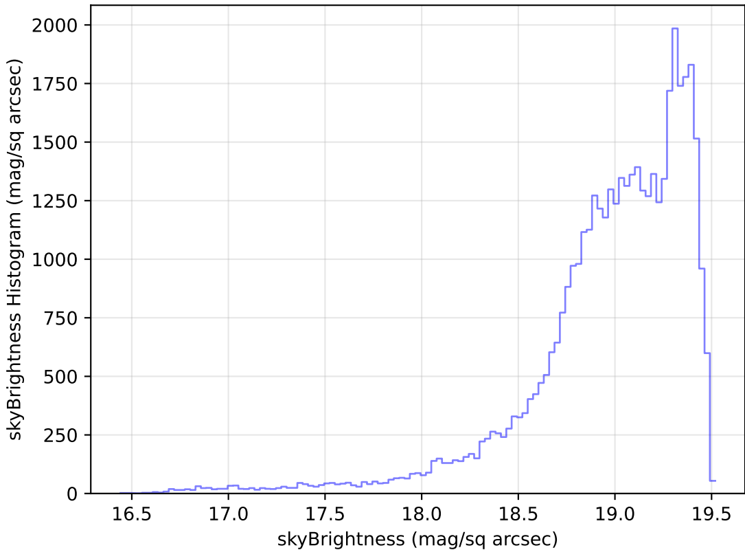
weather_cloudso4v3.4_10yrs Yr 1 z band: skyBrightness Histogram
