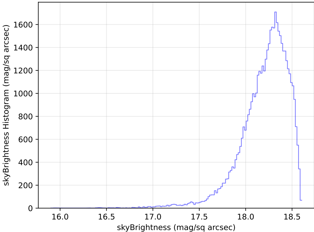
weather_cloudso4v3.4_10yrs Yr 1 y band: skyBrightness Histogram
