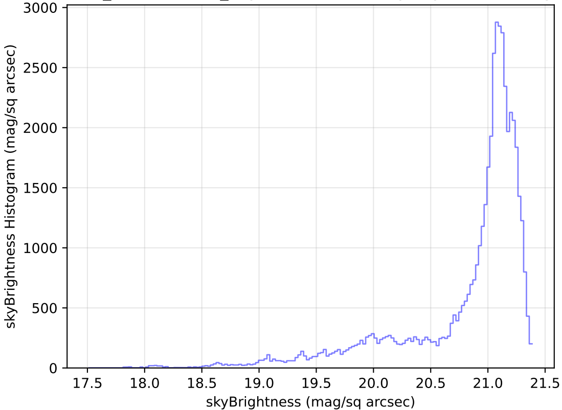
weather_cloudso4v3.4_10yrs Yr 1 r band: skyBrightness Histogram
