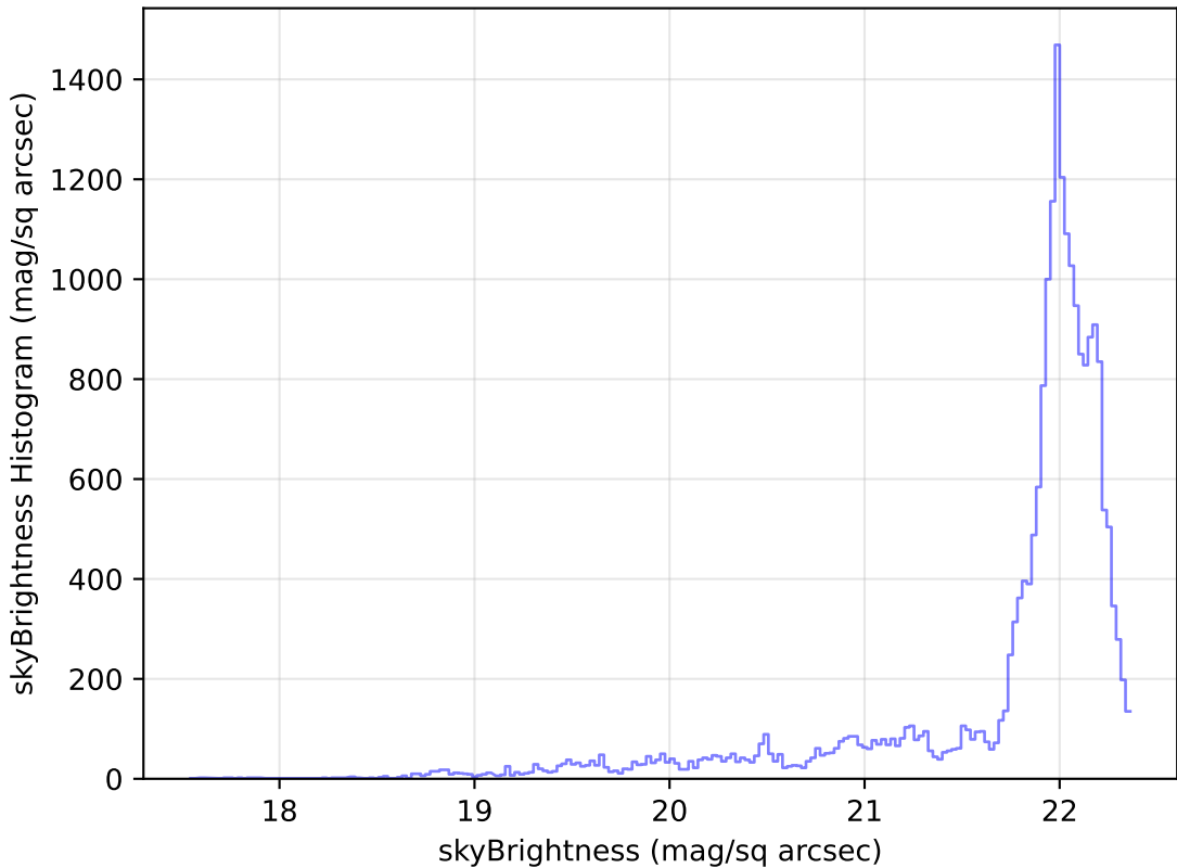
weather_cloudso4v3.4_10yrs Yr 1 g band: skyBrightness Histogram
