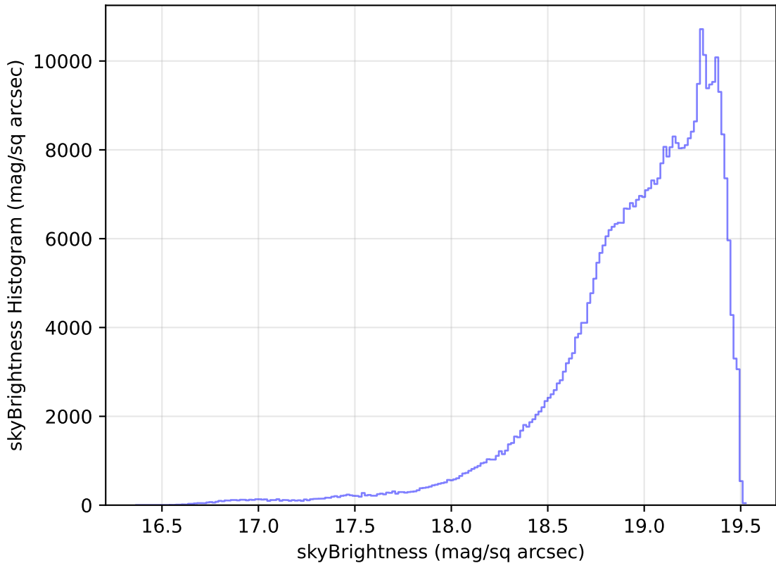
weather_cloudso4v3.4_10yrs WFD z band: skyBrightness Histogram
