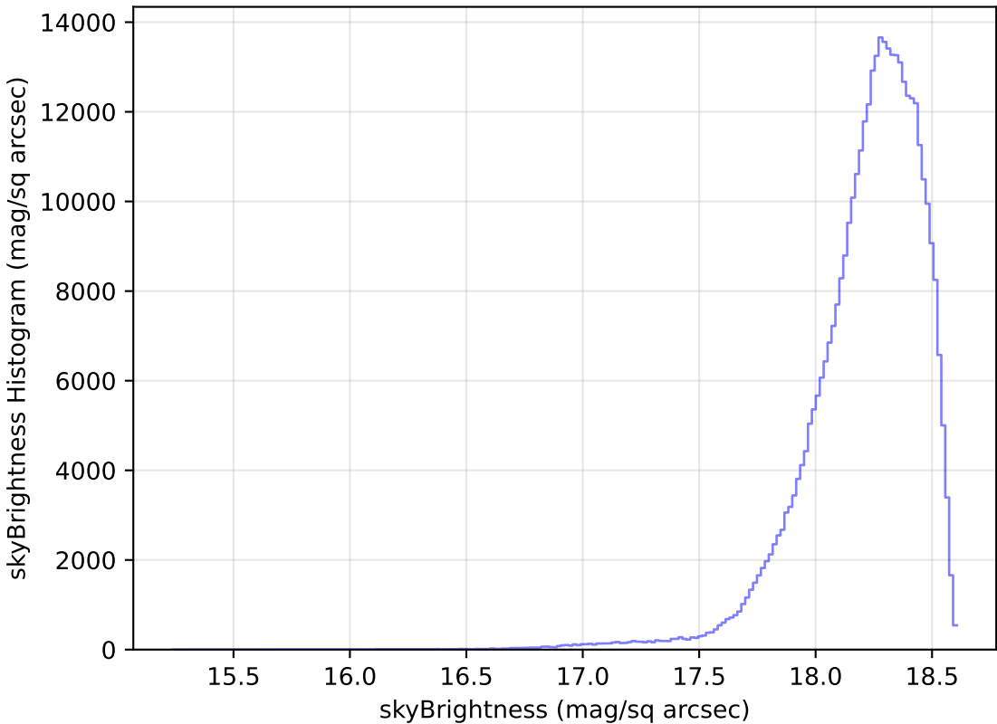
weather_cloudso4v3.4_10yrs WFD y band: skyBrightness Histogram
