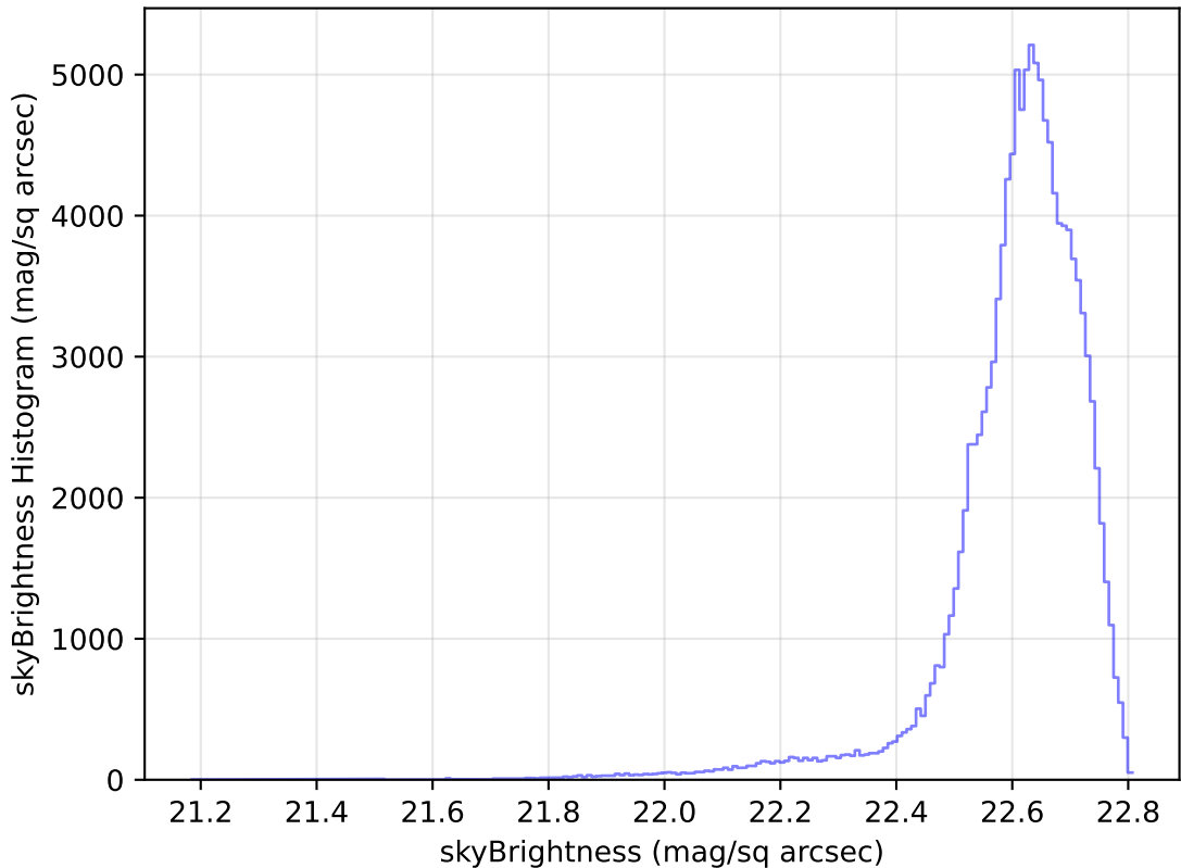
weather_cloudso4v3.4_10yrs WFD u band: skyBrightness Histogram
