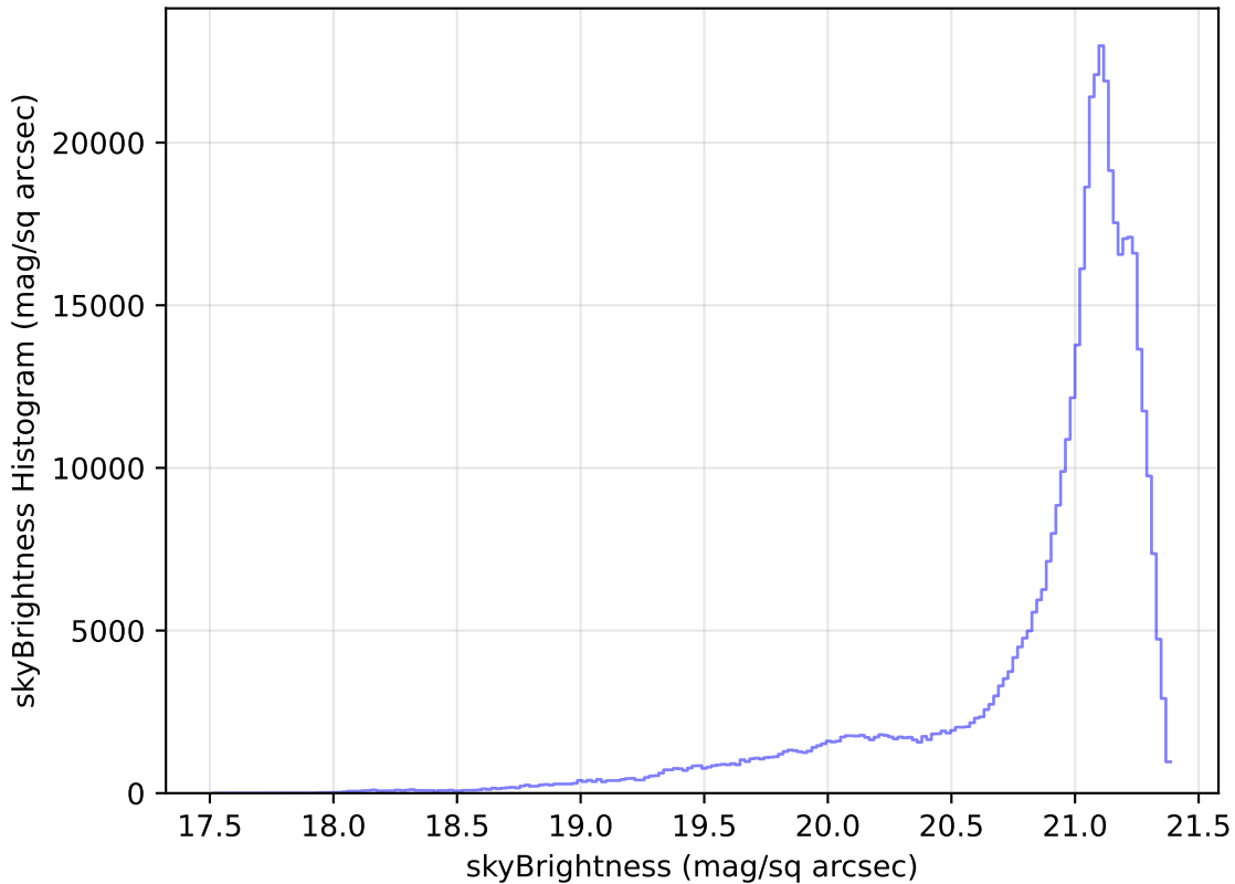
weather_cloudso4v3.4_10yrs WFD r band: skyBrightness Histogram
