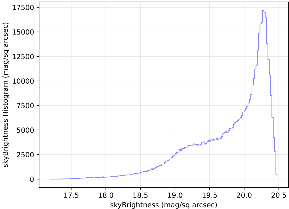
weather_cloudso4v3.4_10yrs WFD i band: skyBrightness Histogram
