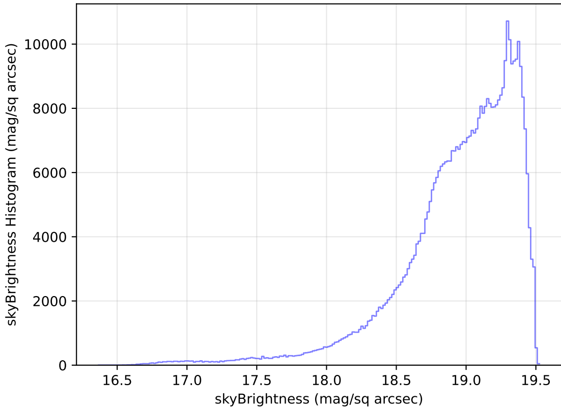
weather_cloudso4v3.4_10yrs All sky z band: skyBrightness Histogram
