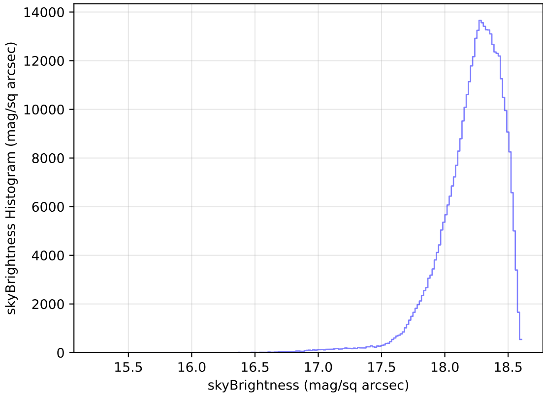
weather_cloudso4v3.4_10yrs All sky y band: skyBrightness Histogram
