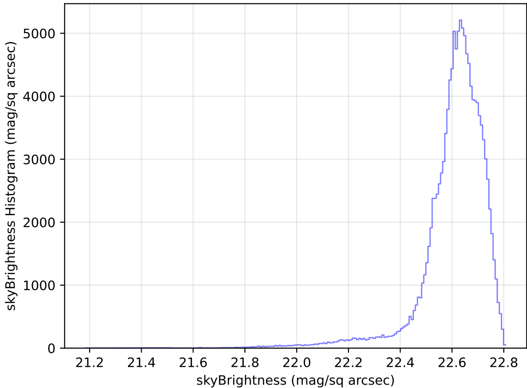
weather_cloudso4v3.4_10yrs All sky u band: skyBrightness Histogram
