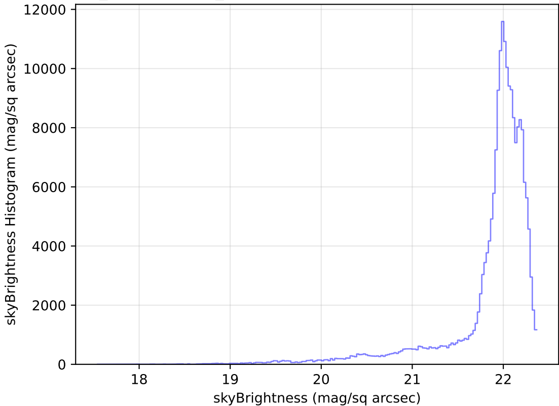
weather_cloudso4v3.4_10yrs All sky g band: skyBrightness Histogram
